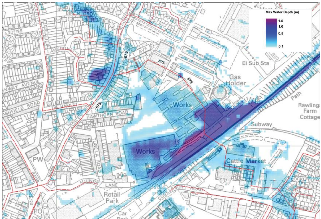
Figure 5-6: Wessex Water surface water sewer location and approximate diameters (in mm) within the vicinity of Langley Business Park. Pluvial modelling results for the 1% AEP rainfall event inclusive of climate change.
