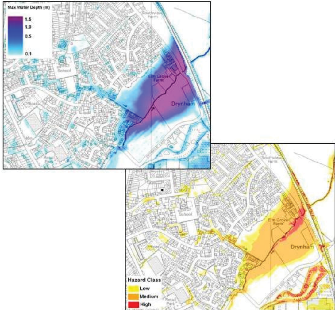
Figure 6-8: Pluvial modelling results (maximum potential depth and hazard) for the 1% AEP rainfall event including an allowance for climate change for the Drynham Road Area.
