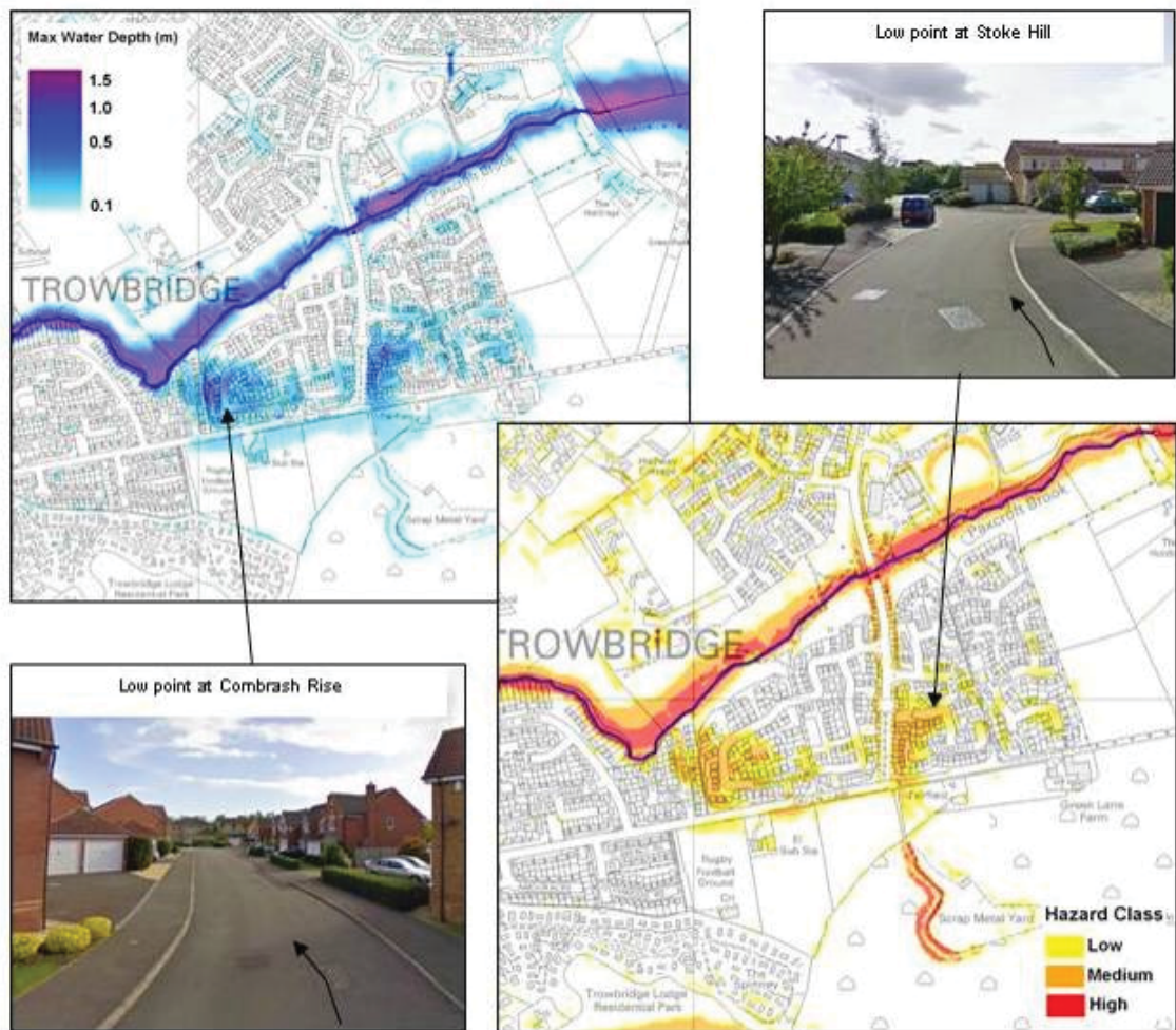
Figure 6-3: Pluvial modelling results (maximum potential depth and hazard) for the 1% AEP rainfall event including an allowance for climate change for the Green Lane Area.
